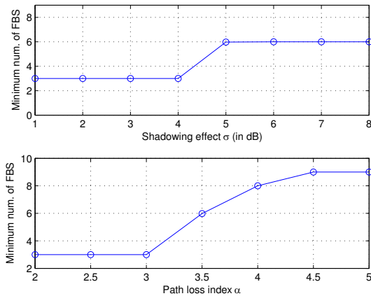
Fig. 8. The scaling of minimum number of FBSs for network coverage as the path loss exponent and the shadowing effect deviation grow.
