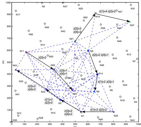
Fig. 7. Scheduling result on each link.
